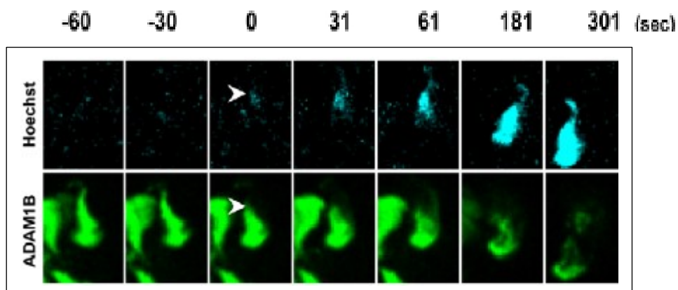
Fig.1 Immunofluorescent staining of ADAM1B during sperm-egg fusion
