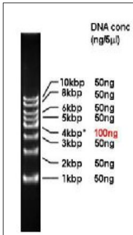
Figure. Electrophoretic pattern of 1 kbp DNA ladders on 1% agarose gel in TAE buffer. Five \mu l of the DNA ladder solution was applied.
