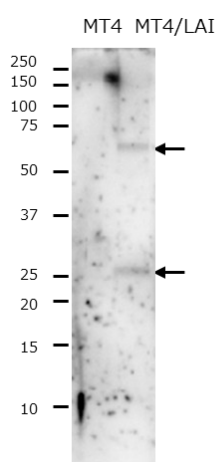
Fig.2 Detection of HIV-1 p24 and precursor proteins p55 and p41 by Western blotting using the anti p24 antibody (65-023).
