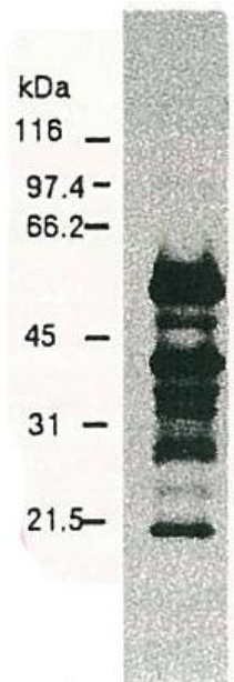
Fig.1 Western blotting of HCV NS5a protein. Chimp liver cells were infected with recombinant vaccinia virus containing a HCV genome cDNA and were subjected to Western blotting using the anti-NS5a antibody. The multitude of NS5a-specific products must be the degraded products of NS5a protein (52 kD).
