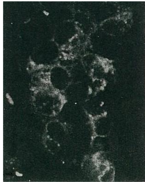
Fig.2 Detection of HCV NS5a protein by immunofluorescence antibody staining. Chimp liver cells were infected with recombinant vaccinia virus containing a HCV genome cDNA. After incubation for 48 hr, the cells were fixed with acetone and HCV NS5a protein was detected by indirect immunofluorescence staining using this antibody.
