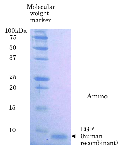
Fig. 1. SDS-PAGE of human EGF'
