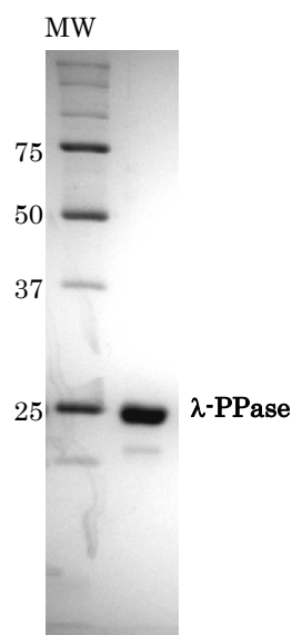
Fig.1 SDS-PAGE of λ -PPase
